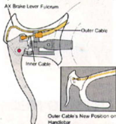
Outer Cable's New Position on Handlebar
